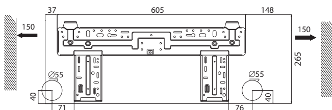
T18H-FS
