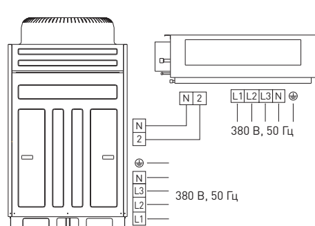
TFR30B, TFR40B
