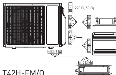
T24H-FM/O2
