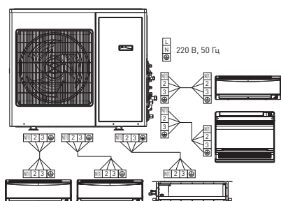
T28H-FM/O, T36H-FM/O
