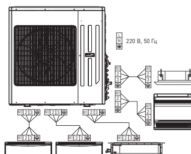
T42H-FM/O
