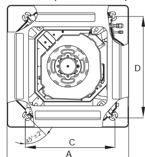
T24H-LC/I—T60H-LC/I
